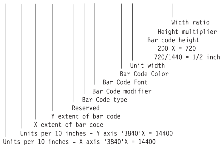
Figure 4. Command format for bar-code commands using CVTDTA (Part 1 of 2)
