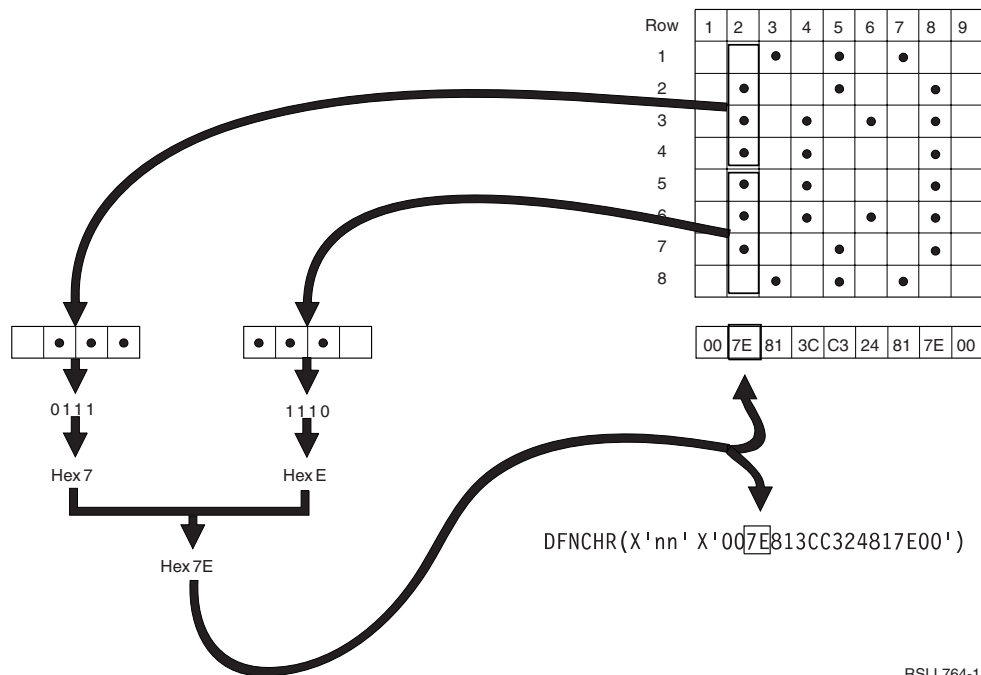
Figure 15. Specify the dot matrix for a copyright mark
