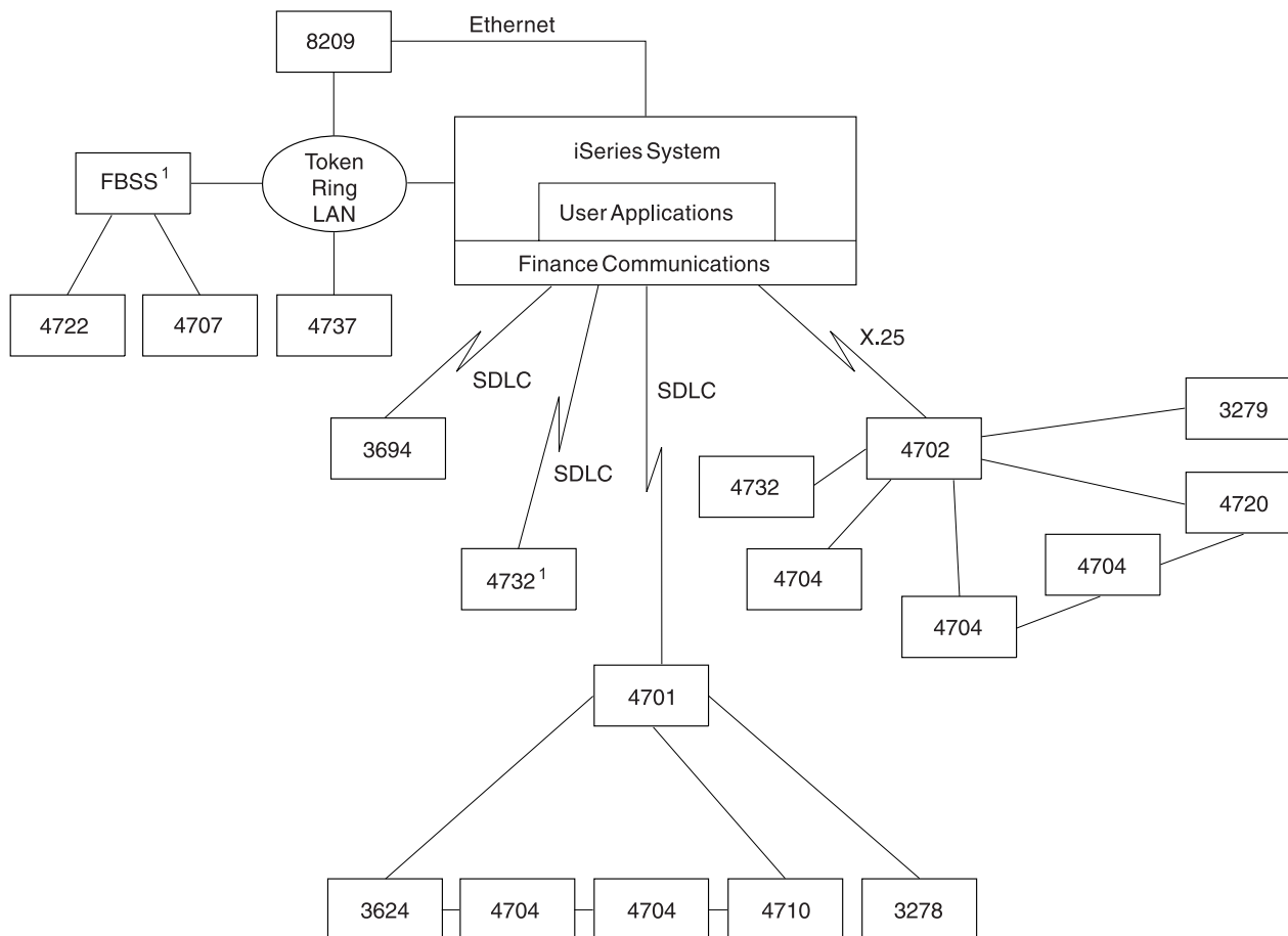
Figure 10. A figure showing the structure of communications between an iSeries server and finance controllers
