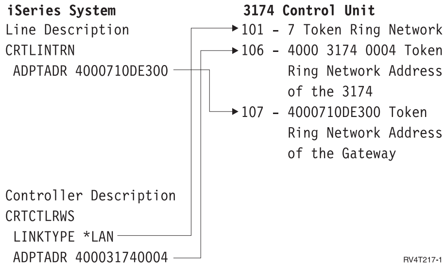
Figure 9. Figure showing the iSeries system parameters and 3174 parameters that need to match when you use token-ring
