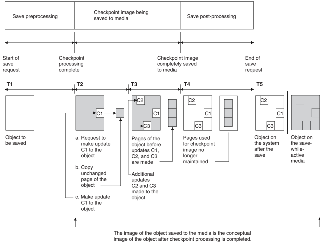
Figure 6. Server management of updates to objects after checkpoint processing is complete
