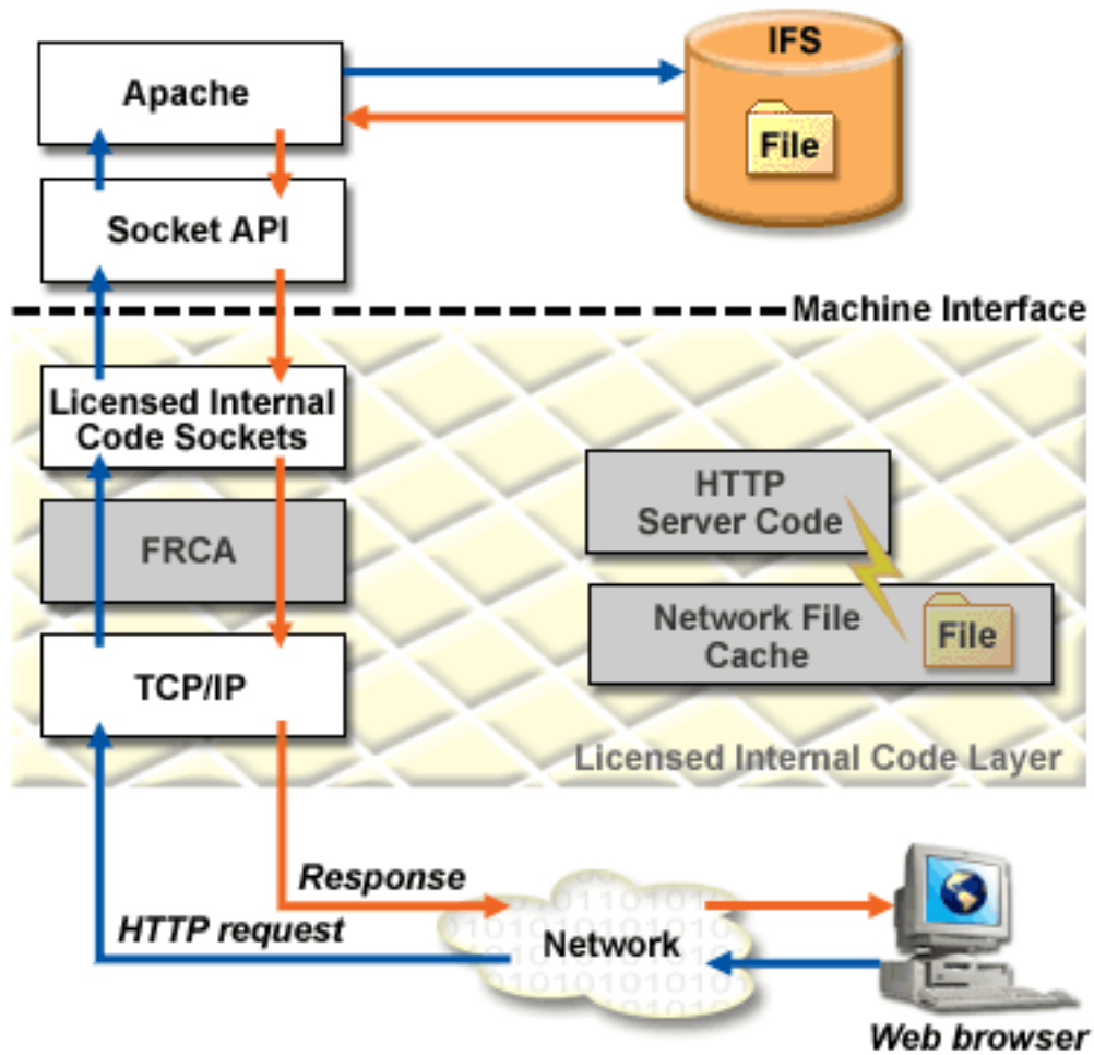
Static content request and response process with FRCA
