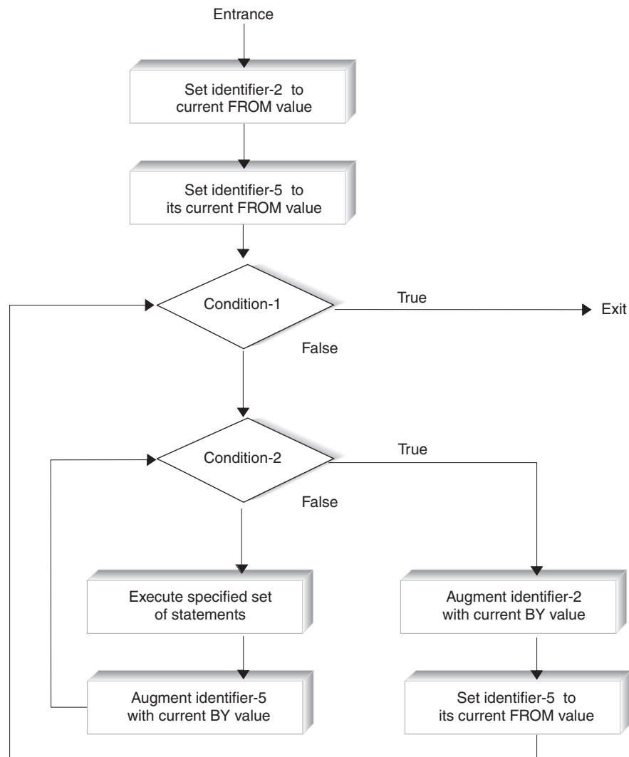
Figure 18. Varying Two Identifiers—with TEST BEFORE
