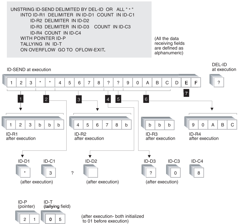
Figure 25. Results of UNSTRING Statement Execution
