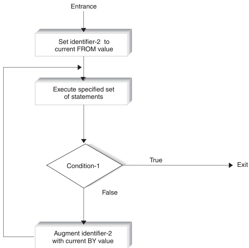
Figure 17. Varying One Identifier—with TEST AFTER
