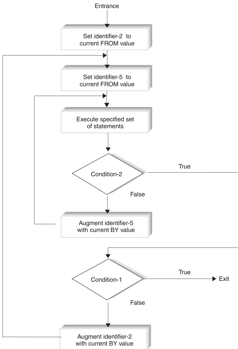
Figure 19. Varying Two Identifiers—with TEST AFTER
