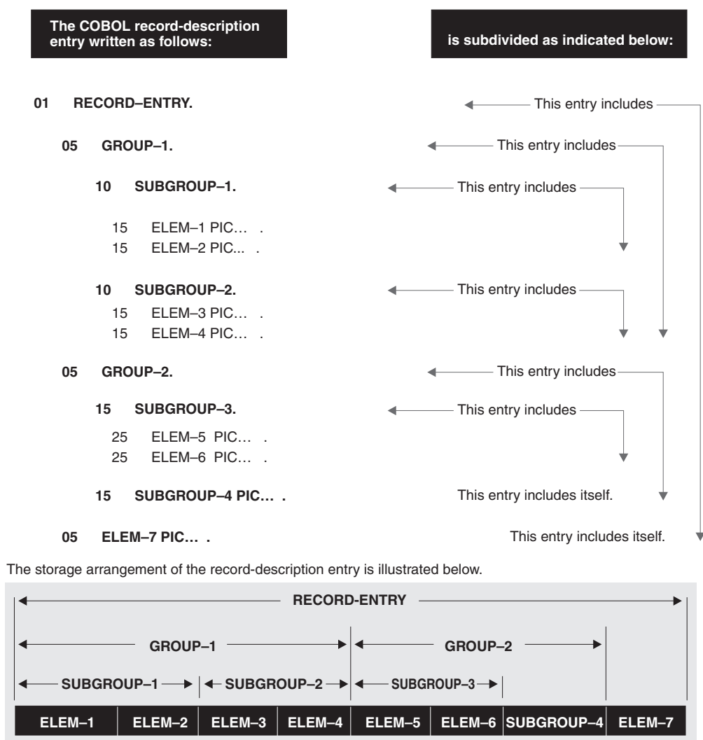
Figure 4. Levels in a Record Description
