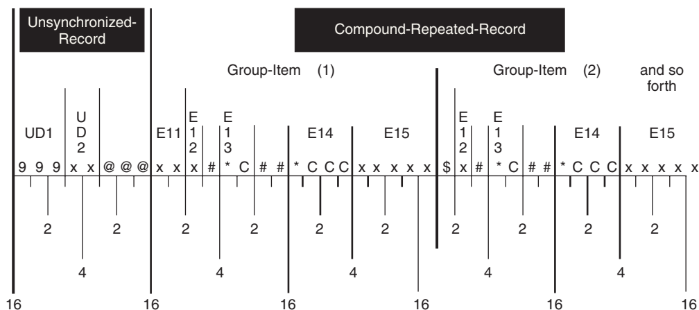
Figure 11. Computer Storage Allocation
