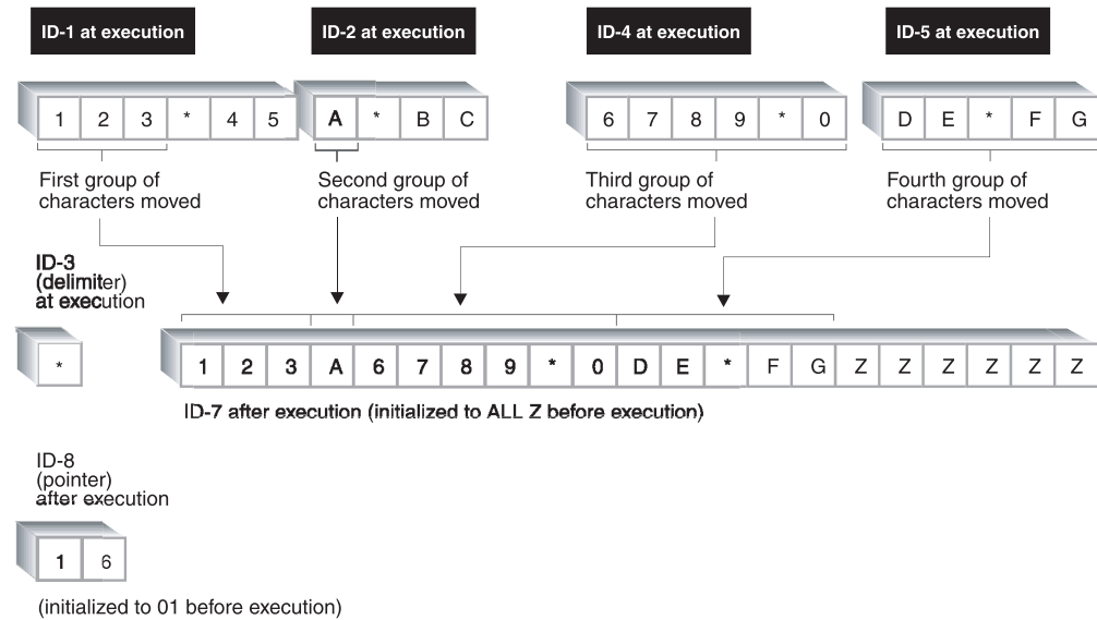
Figure 23. Results of STRING Statement Execution
