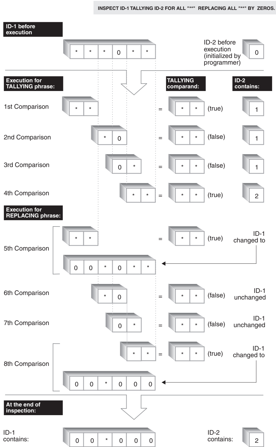
Figure 15. Example of INSPECT Statement Execution Results
