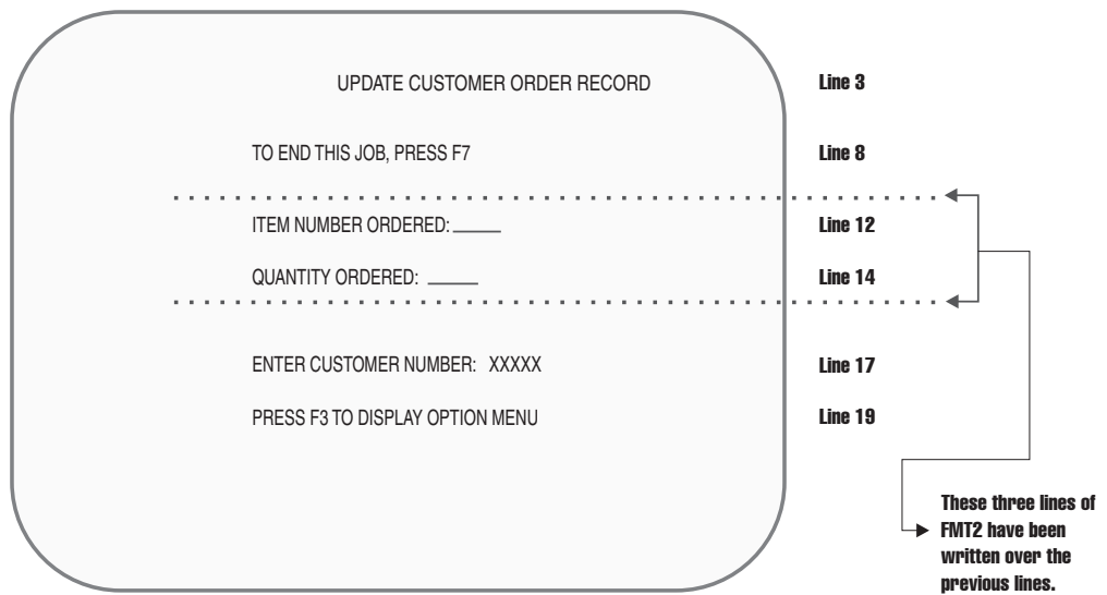
Figure 27. Example of ROLLING Operation
