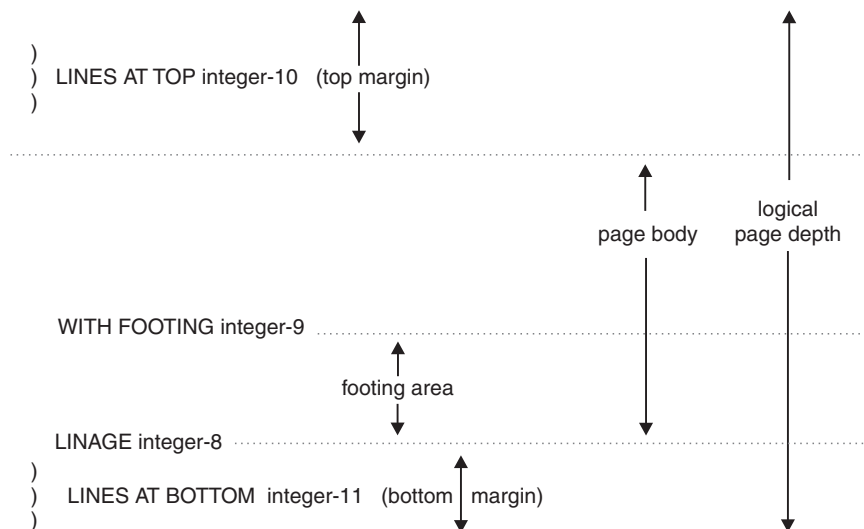
Figure 5. LINAGE Clause Phrases
