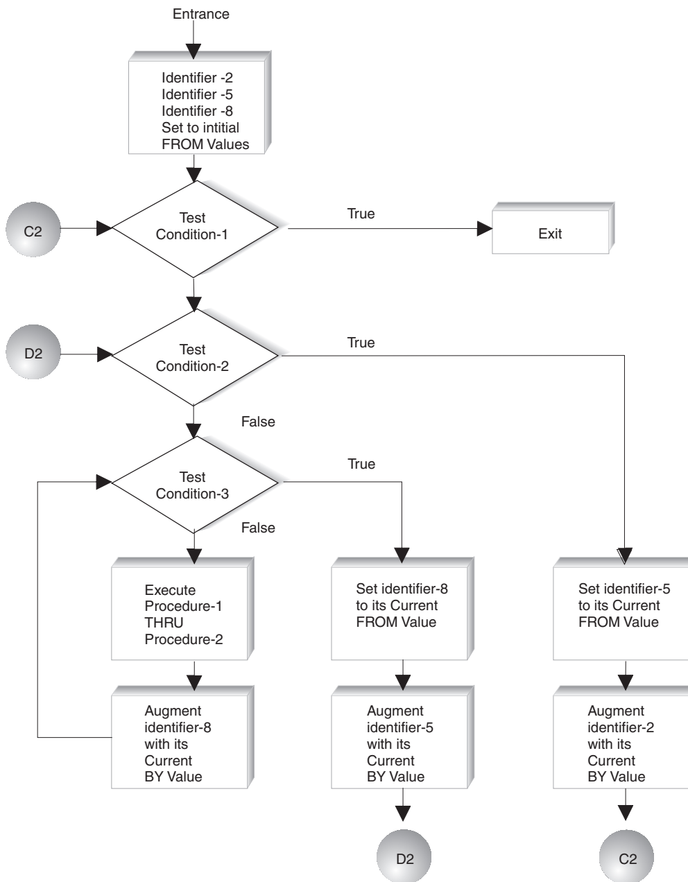
Figure 20. Format 4 PERFORM Statement Logic—Varying Three Identifiers
