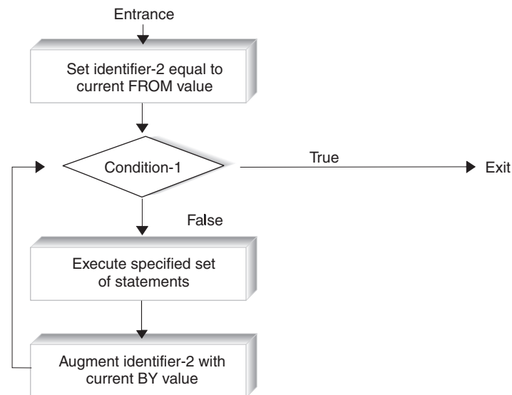
Figure 16. Varying One Identifier—with TEST BEFORE
