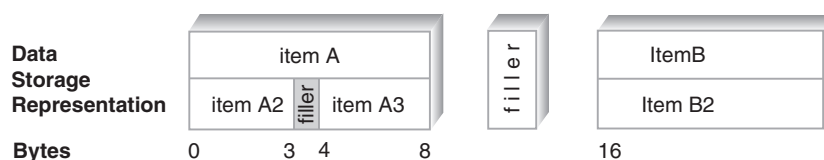
Figure 10. Data Storage Representation Without and With Synchronization
