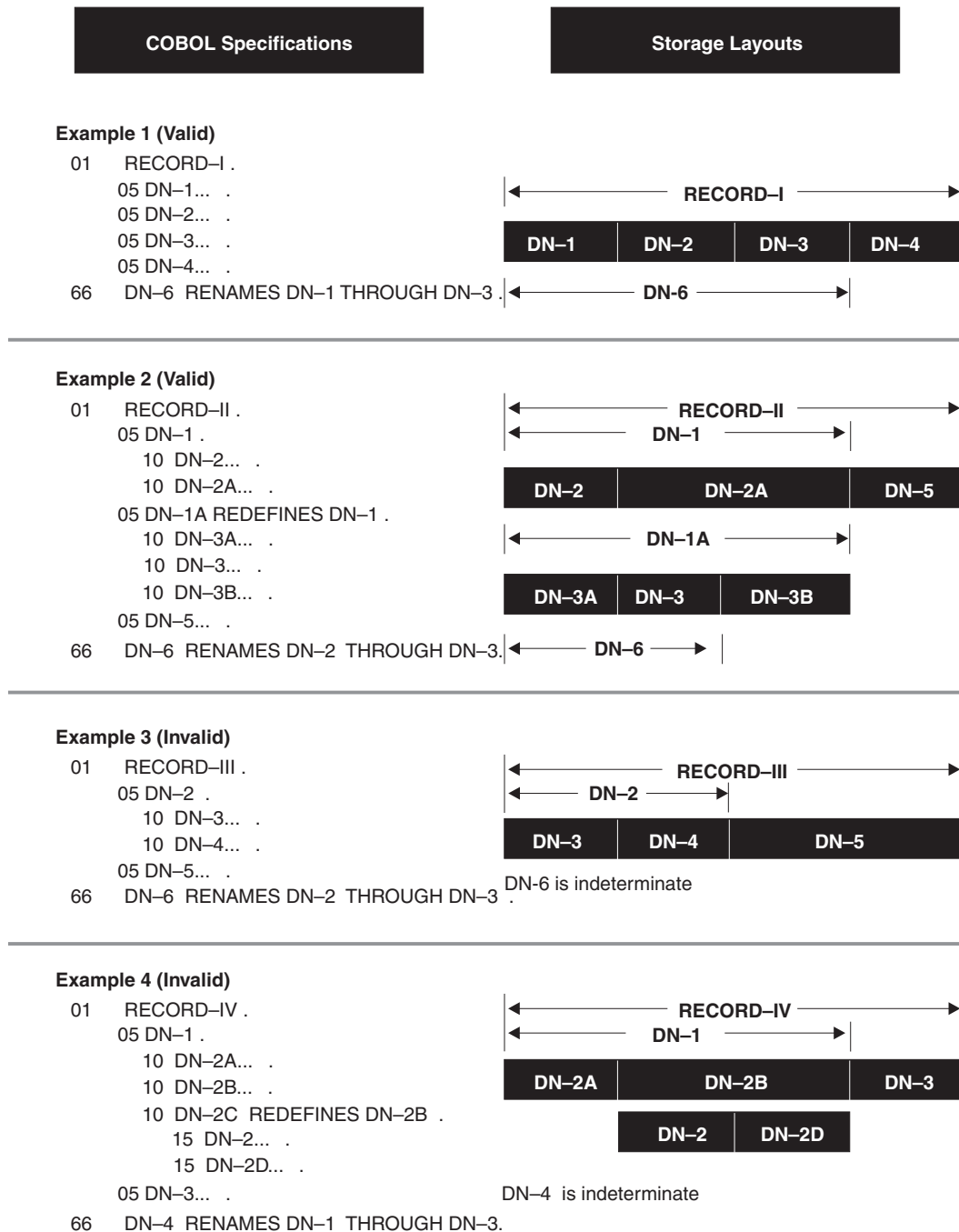
Figure 9. RENAMES Clause—Valid and Invalid Specifications
