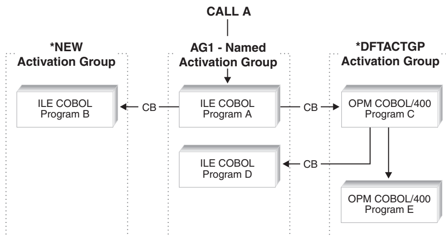
Figure 57. Example of EXIT PROGRAM, STOP RUN, and GOBACK behavior in *NEW, Named, and *DFACTGTP Activation Groups
