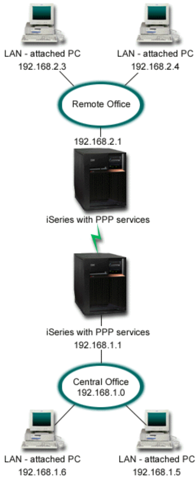
Figure 6. Connect your corporate and remote networks with a modem
