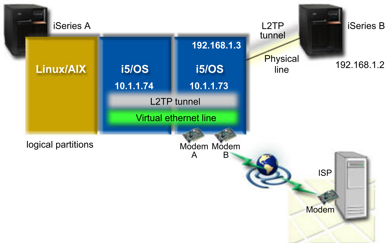
Figure 9. Multiple systems sharing the same modem for dial-up connections
