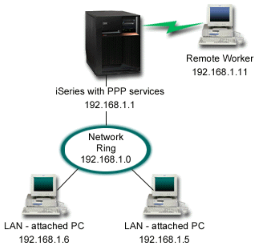
Figure 4. Connect remote clients to your iSeries server
