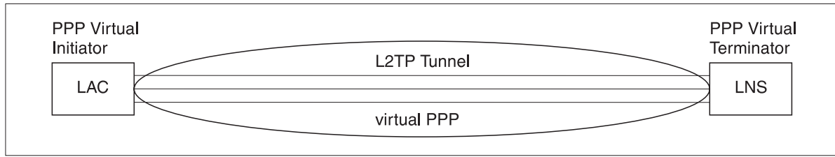
Figure 10. PPP virtual initiator or PPP virtual terminator
