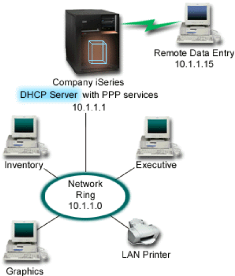
Figure 1. PPP and DHCP on a single iSeries server
